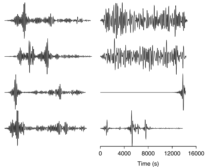
Figure 3. As Fig. 2, but for the mantle-wave class. Again, left-hand column contains plausible traces; right-hand column traces are unusable.
