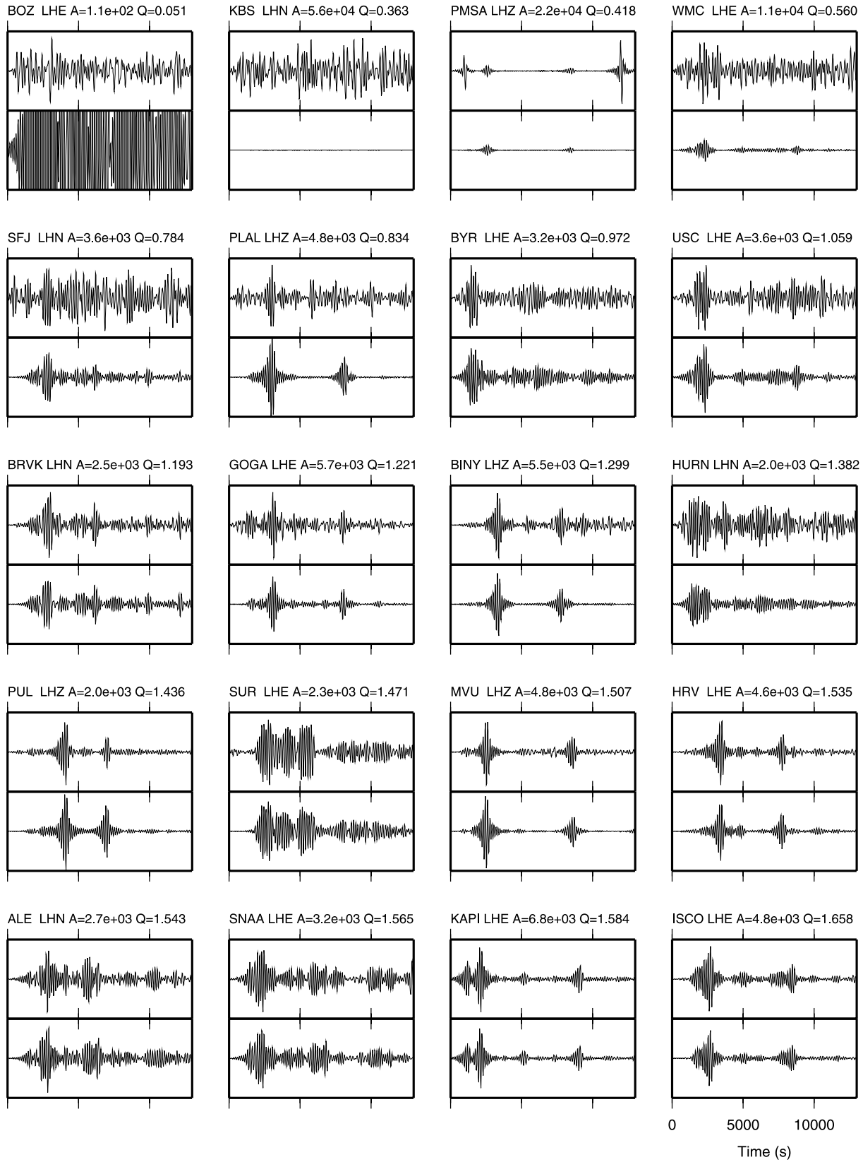
Figure 12. Sample mantle-wave traces (top panels) and corresponding synthetics (bottom panels) from event 010800G, arranged in ascending order of network-assigned quality factor (Q), defined as in eq. (26). All traces are scaled by the maximum data amplitude (A); synthetics are plotted on same scale as the data. Timescales in all panels are identical.
